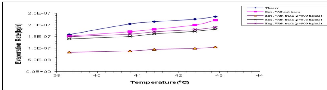
Figure (2) Variation of Evaporation Rate with Temperature
