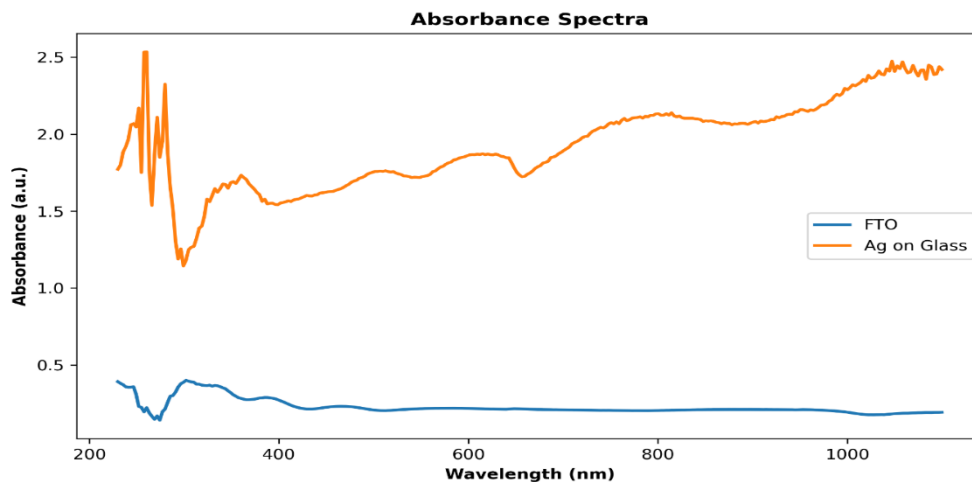
Figure 4: Absorbance spectra of the FTO and Ag thin Film
