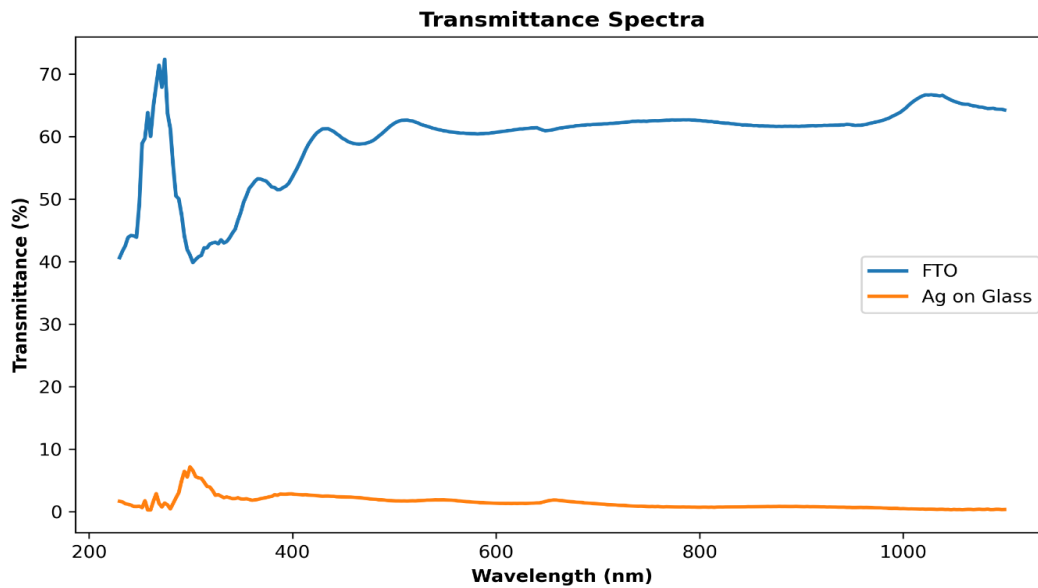
Figure 5: Transmittance spectra of the FTO and Ag thin Film
