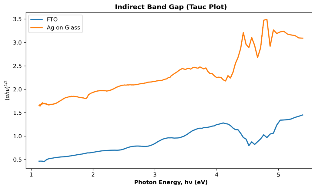
Figure 7: Indirect band-gap of the FTO and Ag thin Film
