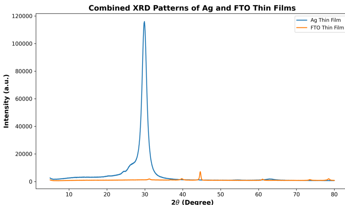
Figure 1: XRD structural characterization results of FTO and Ag thin films
