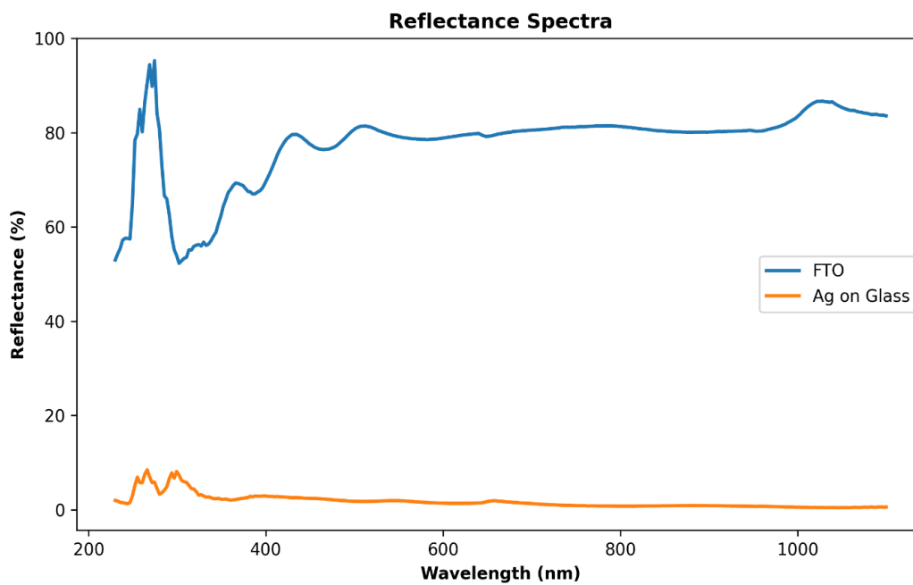
Figure 6: Reflectance spectra of the FTO and Ag thin Film
