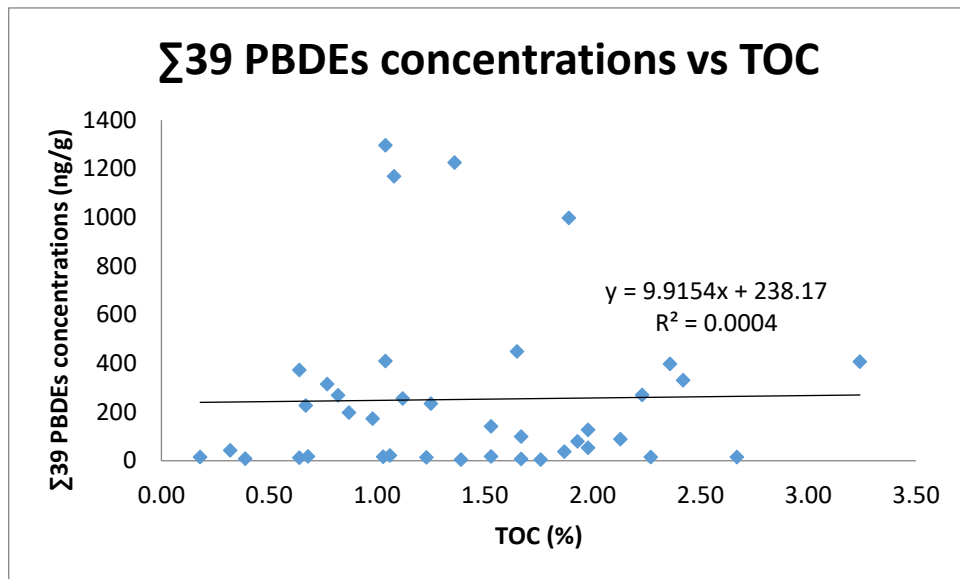
Figure 4.8: Plot of TOC versus the concentrations of the \Sigma 39 PBDEs
